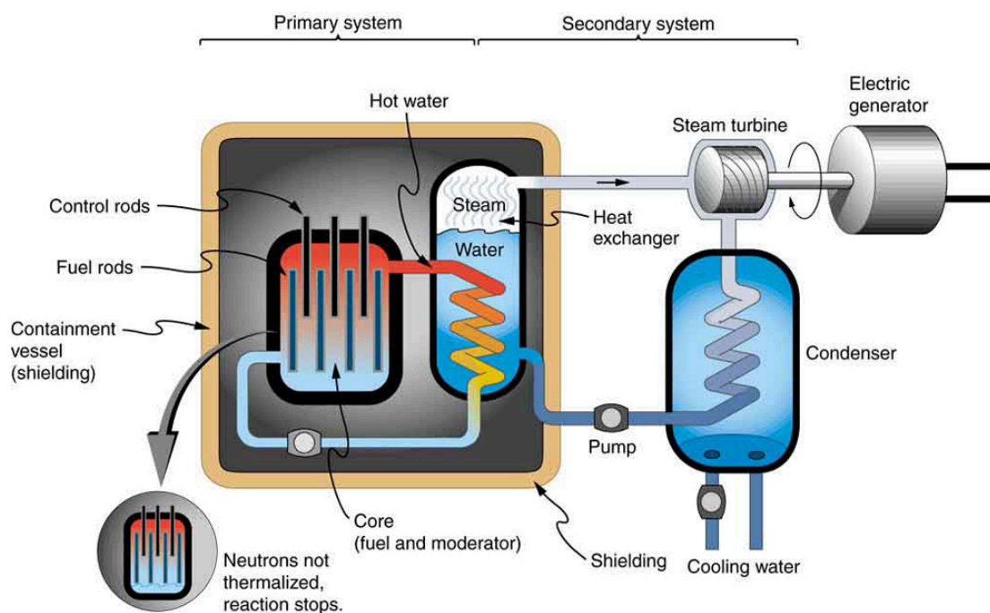
Figure 32.25 A pressurized water reactor is cleverly designed to control the fission of large amounts of ^{235}\text{U} , while using the heat produced in the fission reaction to create steam for generating electrical energy. Control rods adjust neutron flux so that criticality is obtained, but not exceeded. In case the reactor overheats and boils the water away, the chain reaction terminates, because water is needed to thermalize the neutrons. This inherent safety feature can be overwhelmed in extreme circumstances.
