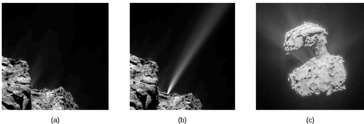
Figure 13.25 Gas Jets on Comet 67P. (a and b) Jet activity was photographed by the Rosetta spacecraft near perihelion. You can see a jet suddenly appearing; it was active for only a few minutes. (c) This spectacular photo, taken near perihelion, shows the active comet surrounded by multiple jets of gas and dust. (credit a, b: modification of work by ESA/Rosetta/MPS; credit c: modification of work by ESA/Rosetta/NAVCAM)
