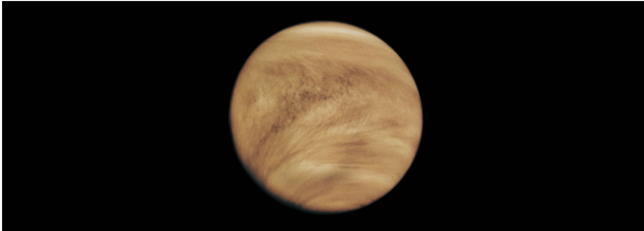
Figure 10.2 Venus as Photographed by the Pioneer Venus Orbiter. This ultraviolet image shows an upper-atmosphere cloud structure that would be invisible at visible wavelengths. Note that there is not even a glimpse of the planet's surface. (credit: modification of work by NASA)
